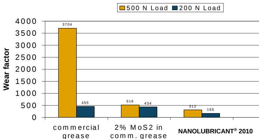
Commercial Grease: Wear Factor - SRV Test
